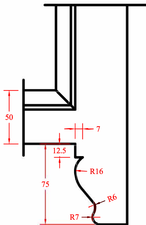
No.2 Horn
