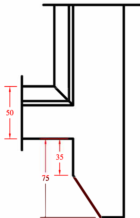
Bevelled Horn
