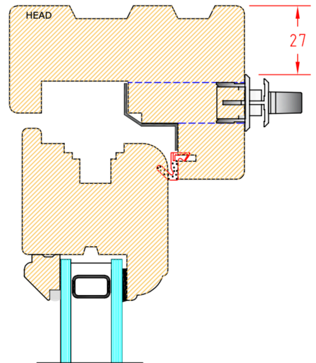
Concealed Head Ventilation
