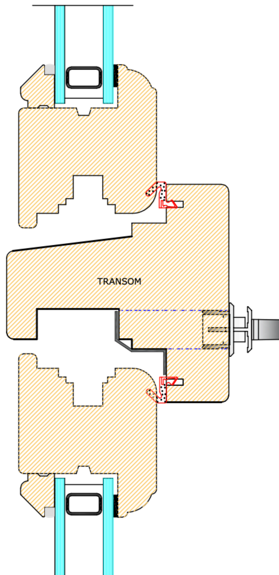
Concealed Transom Ventilation
