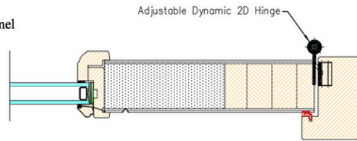
Adjustable Dynamic 2D Hinge
