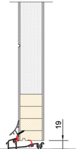
Low Level Threshold Zero Projection
