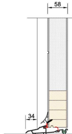
Low Level Threshold 34mm Projection
